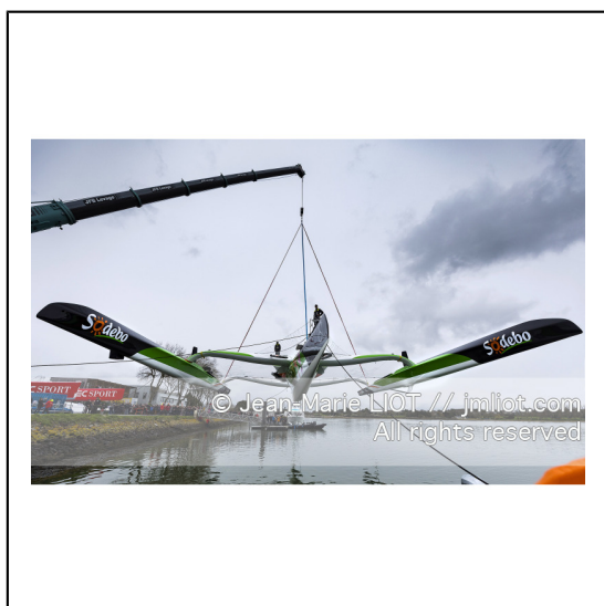
Mise à l'eau du nouveau Sodebo Ultim 3, skipper Thomas Coville, chantier Multiplast Vannes, le 18 mars 2019, photo Jean-Marie LIOT.###.Launching new Sodebo Ultim 3, skipper Thomas Coville, Multiplast shipyard in Vannes (France), on march 18 2019, Photo Jean-Marie LIOT
